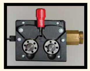
TRAINAFILO A 4 RULLI INGRANATI D. 37 WIRE FEEDER WITH 4 GEARED ROLLERS D. 37
